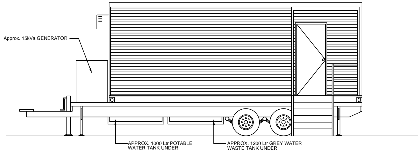
7.2x2.4m Mobile Crib Room - Front Elevaion
