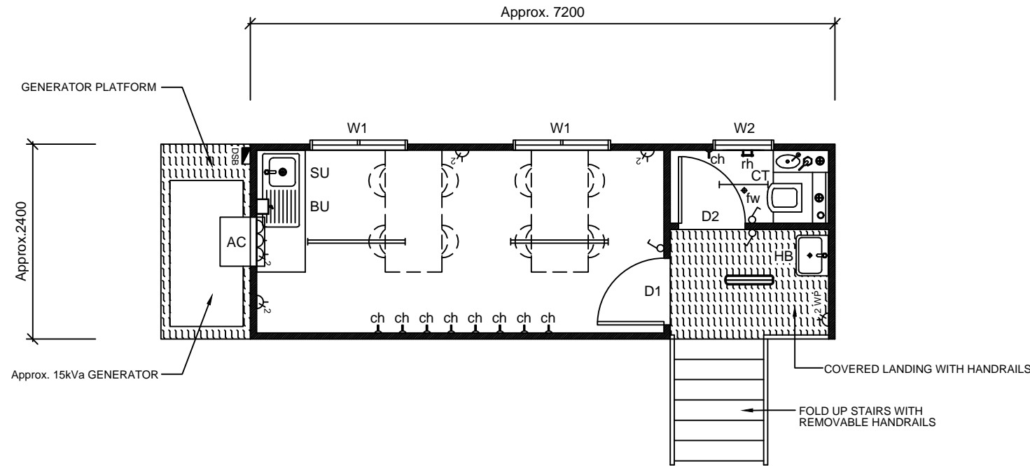
7.2x2.4m Mobile Crib Room - Floor Plan
