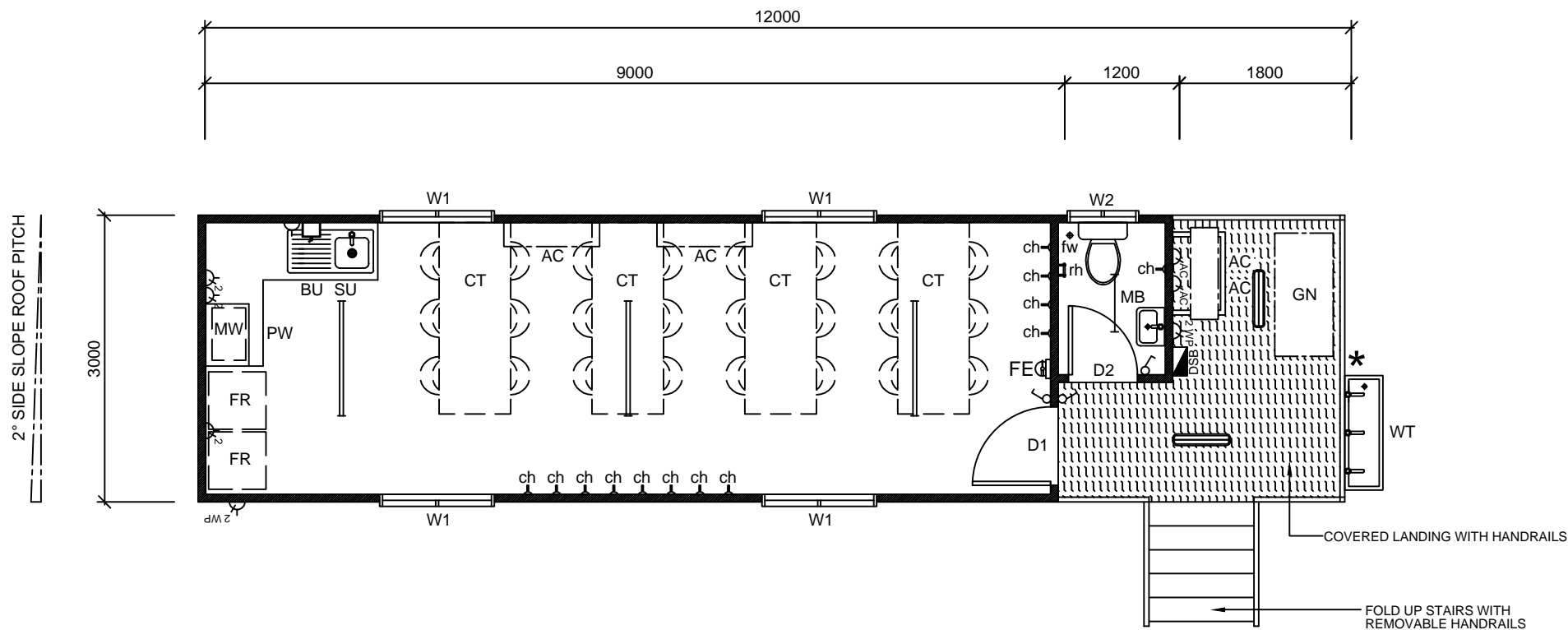
12.0x3.0m Mobile Crib Room - Floor Plan
