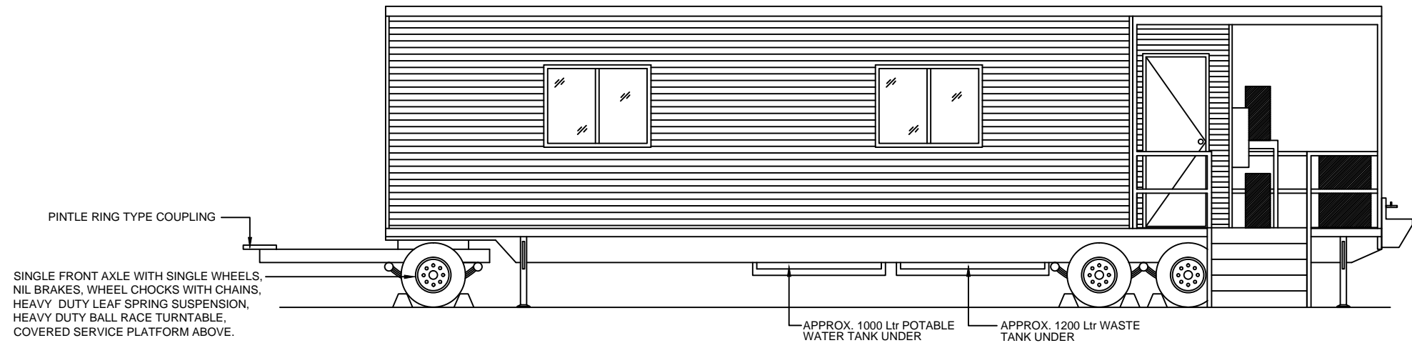
12.0x3.0m Mobile Crib Room - Front Elevation
